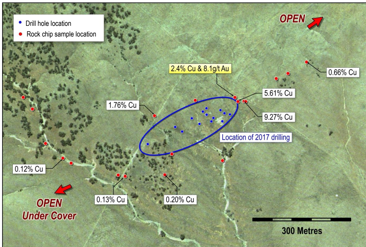
Figure 1: Blue Hills copper project showing location of some rock chips reported in this announcement (red dots) and location of drill collars from recent RC drilling by Archer (blue dots).
