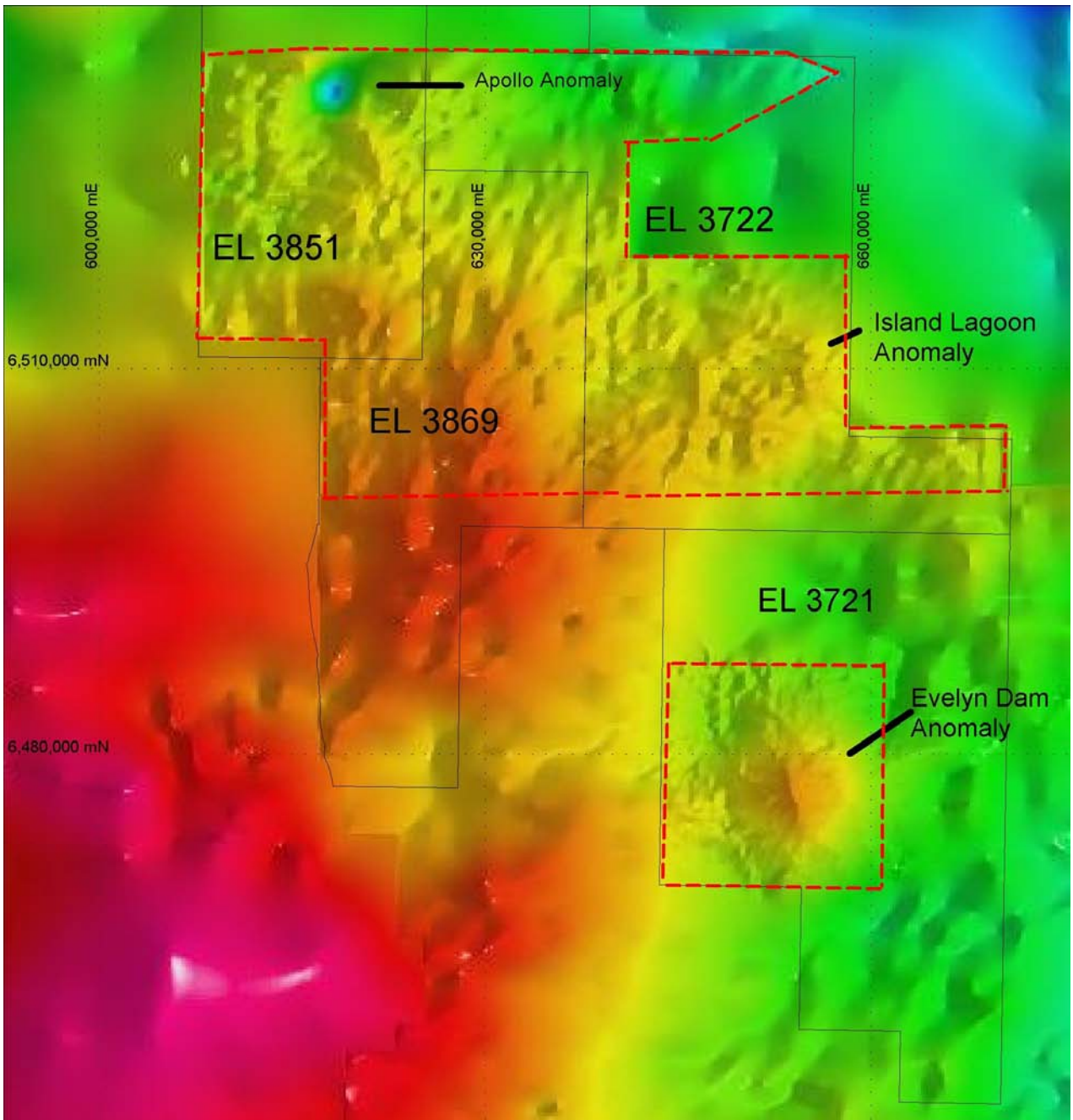
Figure 1: West Roxby Project gravity image and location of drill targets.
